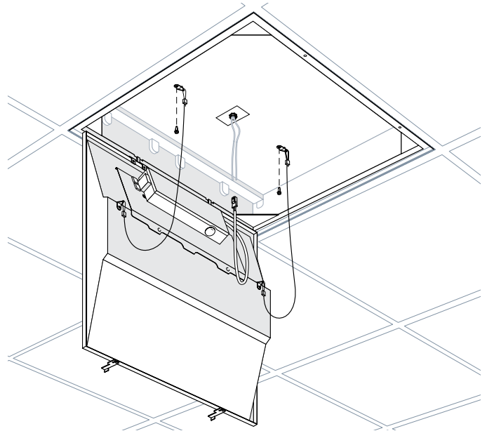
2' x 2' Fixture Hangs From Frame For Easy Wiring
